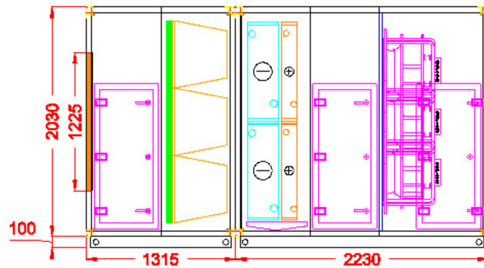
Right View
